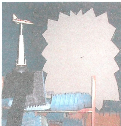
Compact Range RCS Test Facility
