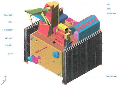
OCEANSAT-2
