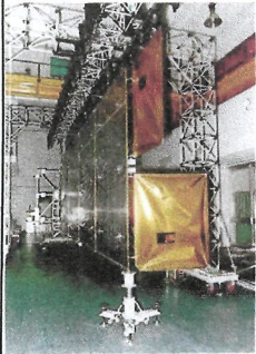
SMA actuated Flap mechanism
