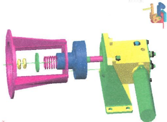
Paraffin release mechanism
