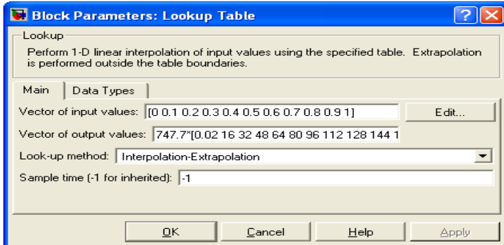
Figure.2. Inclusion of 1-D Power Lookup Table in the Piston Engine Block.
