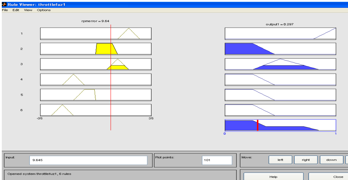
Figure.11. Rule Viewer For Engine RPM To Throttle Fuzzy Logic Controller.
