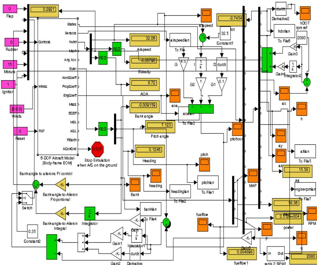
Figure.6. Simulink model for the landing phase of the UAV.
