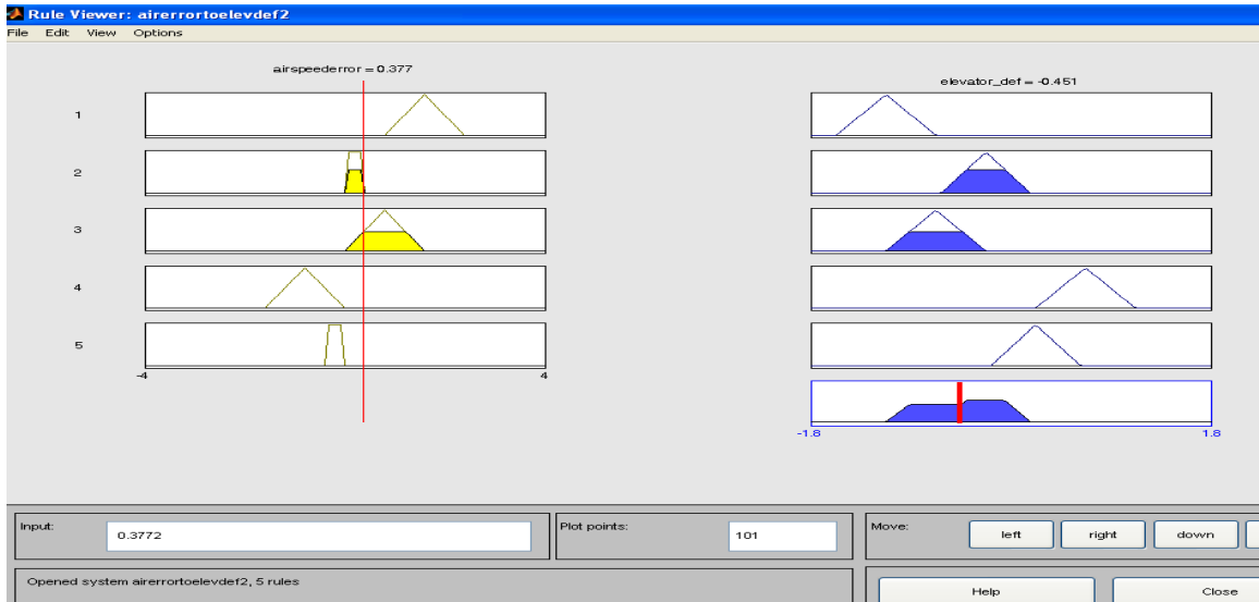
Figure.10. Rule Viewer for Airspeed to Elevator Fuzzy Logic Controller
