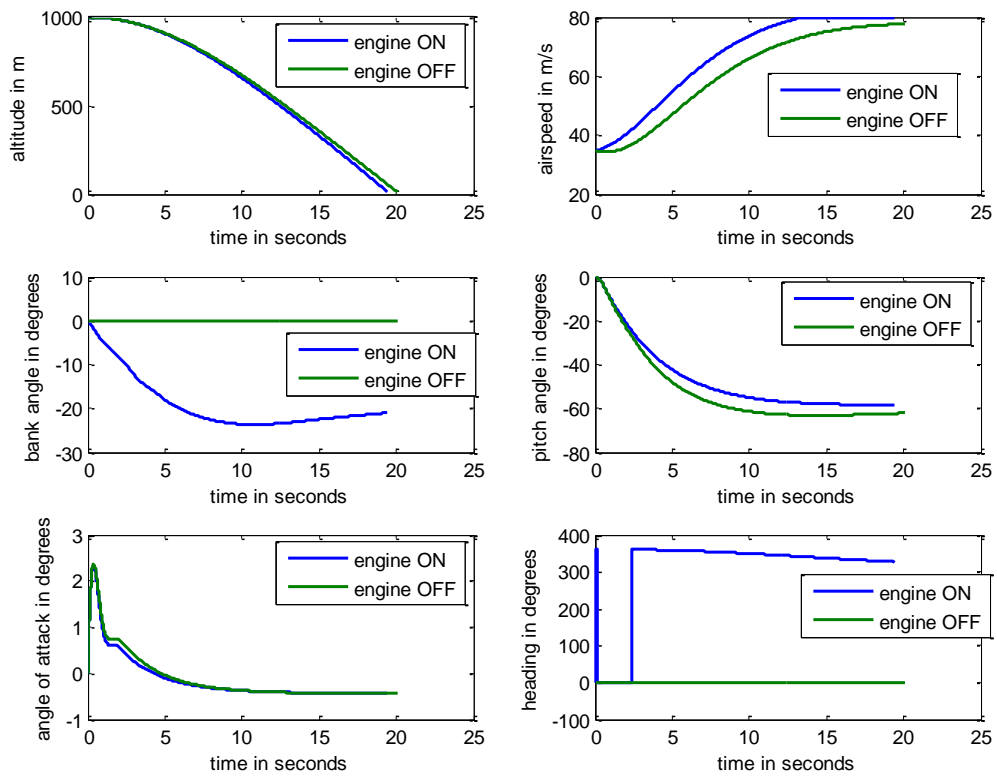
Figure.4. Open loop responses for the UAV model with engine ON and OFF.
